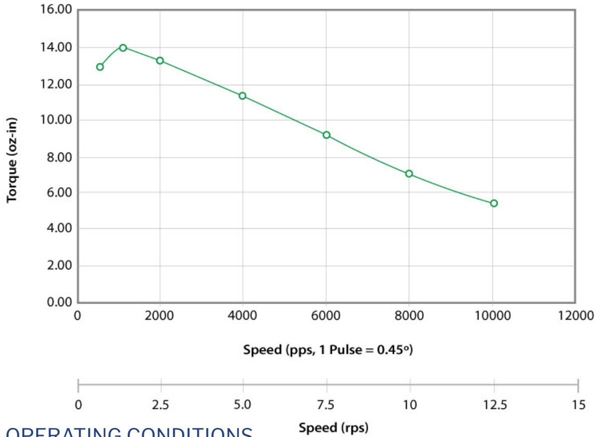
ZH417-11-09 (0.9° Step Motor) 24VDC, 0.8 Amp/Phase, Bipolar, 1/2 Stepping
